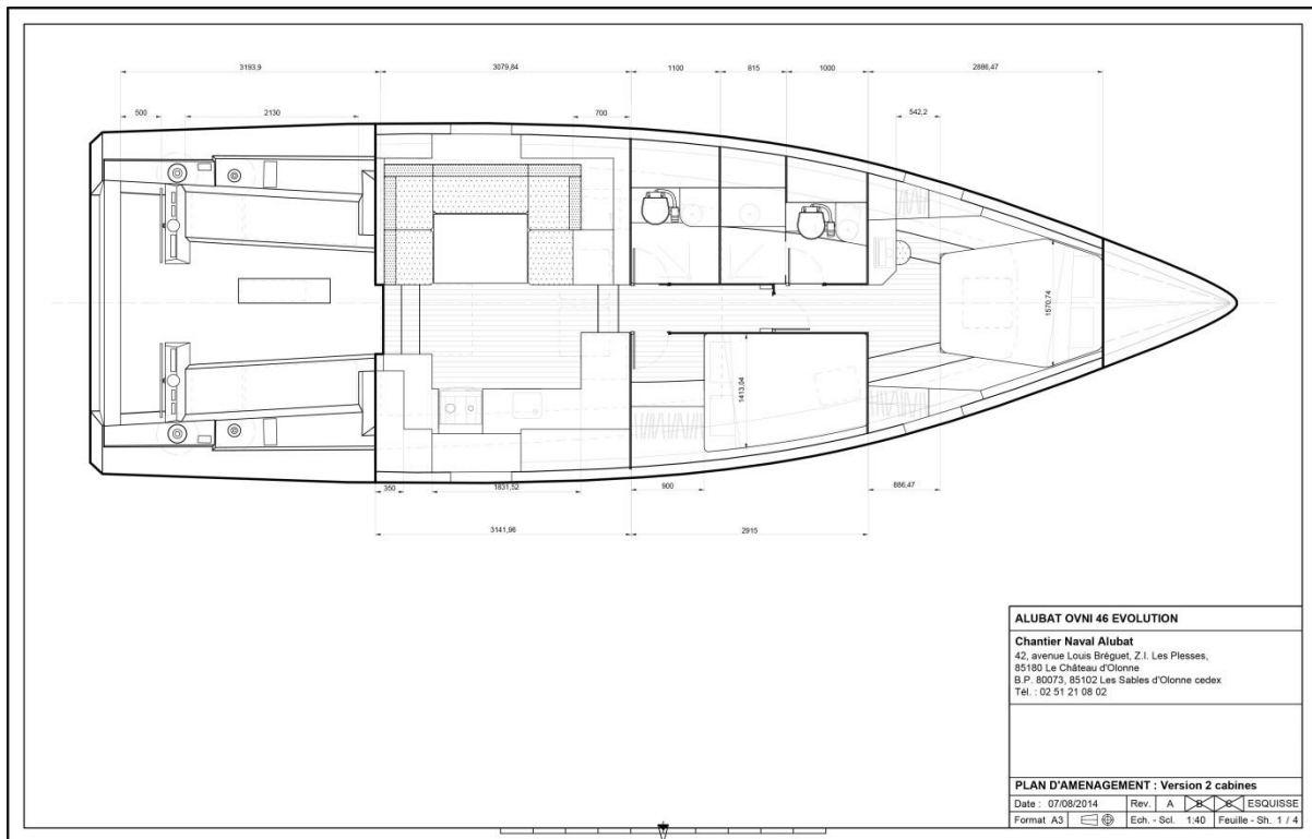
Standard layout – 2 cabins
