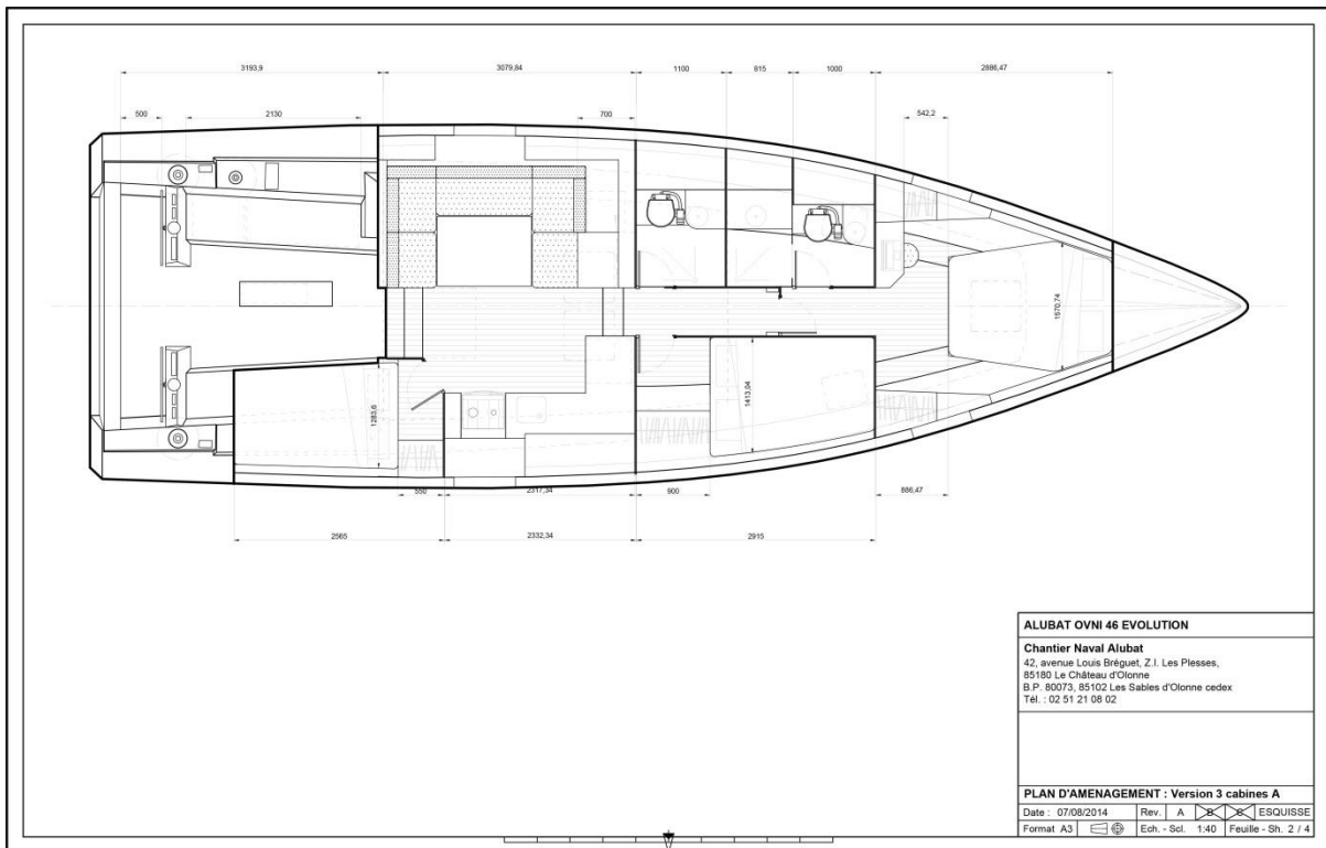
Optional 3 cabin layout – 3 rd cabin aft
