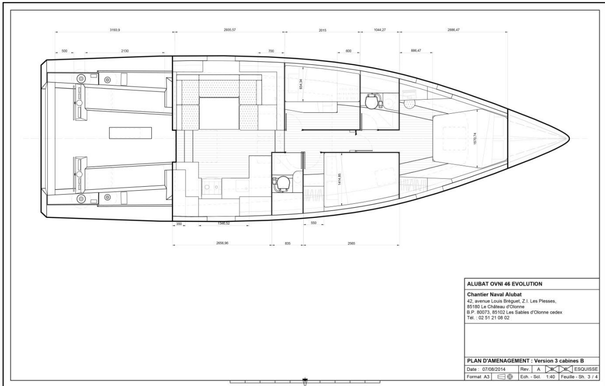
Optional 3 cabin layout – 3 rd cabin forward
